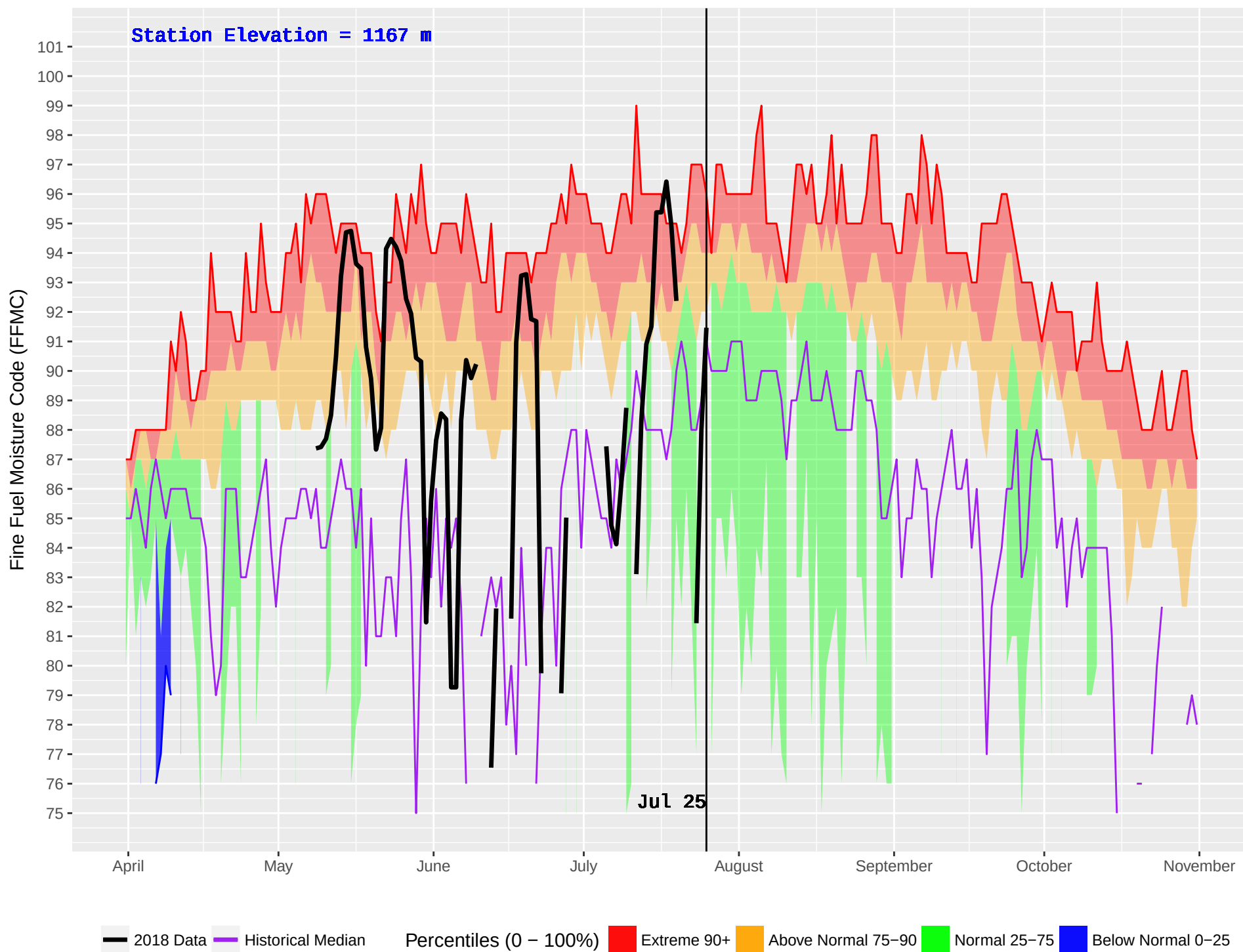
LEIGHTON LAKE (307) : Historical (1982–2016) and Current (2018) Noon Fine Fuel Moisture Code (FFMC)
