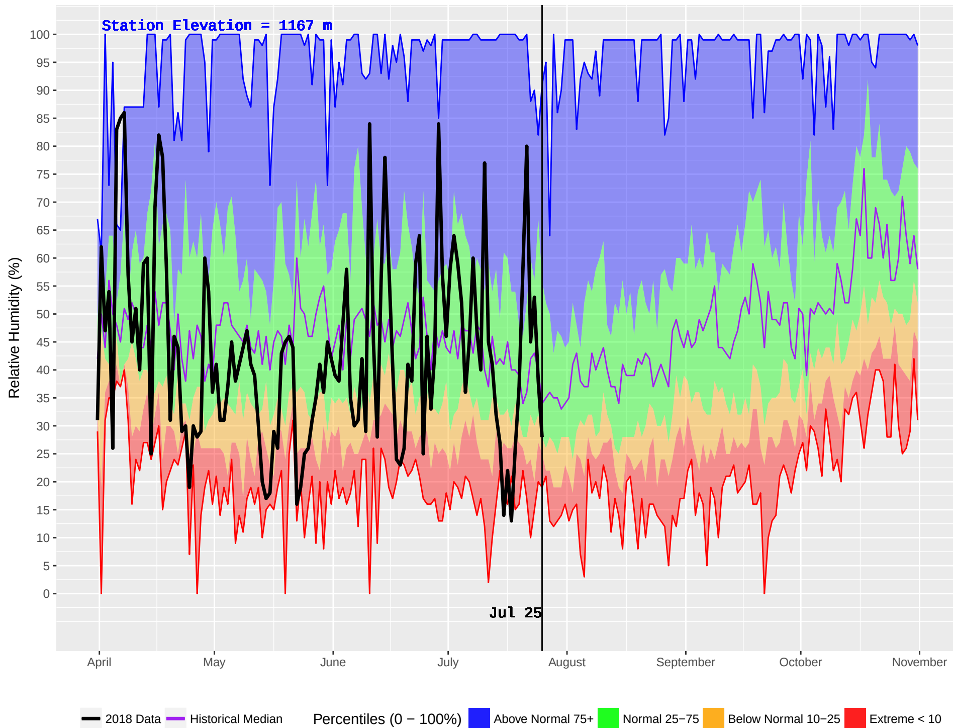
LEIGHTON LAKE (307) : Historical (1982–2016) and Current (2018) Noon Relative Humidity
