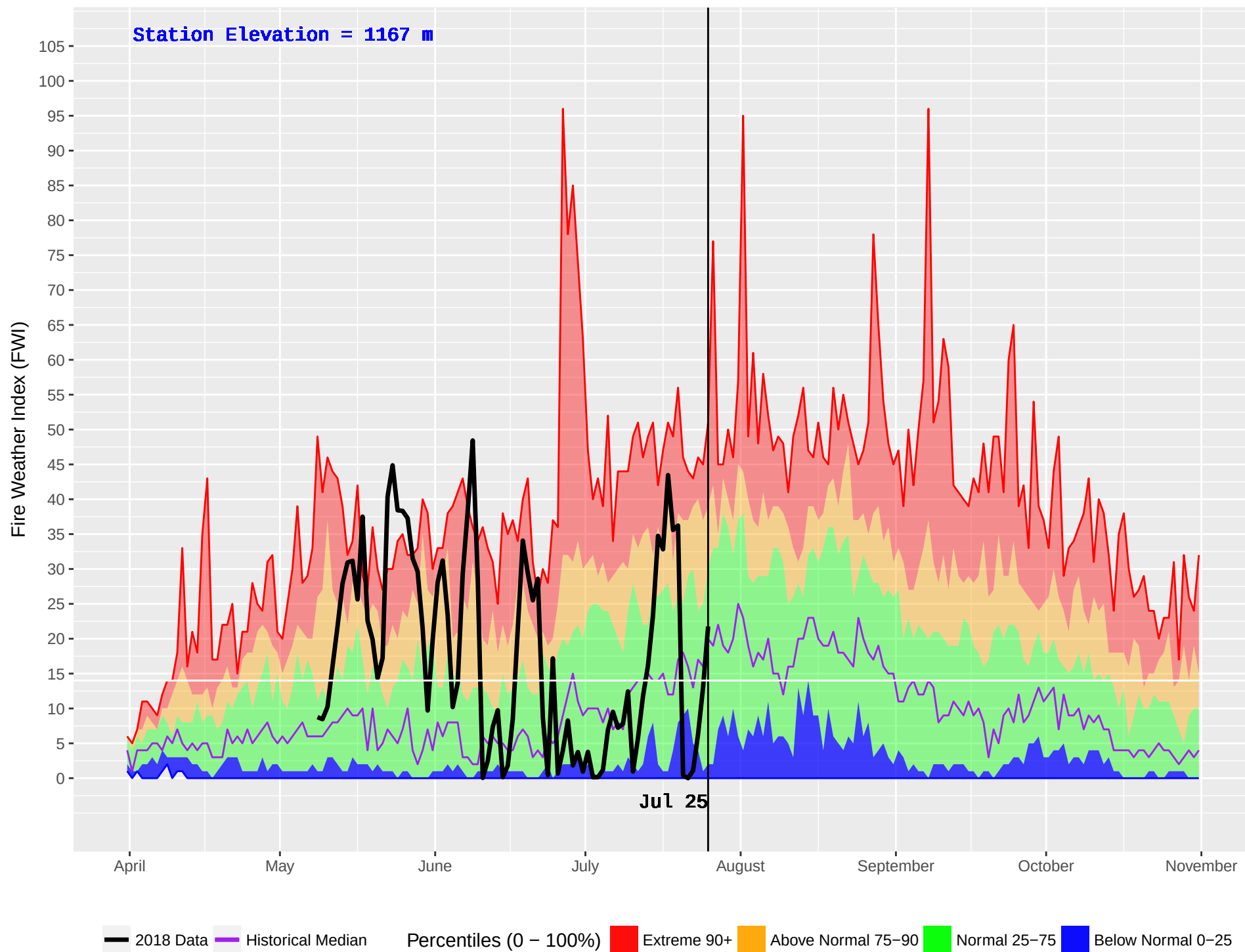
LEIGHTON LAKE (307) : Historical (1982–2016) and Current (2018) Noon Fire Weather Index (FWI)
